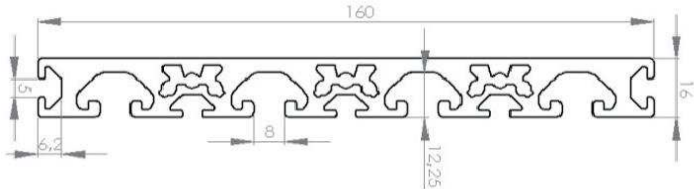
Profile 160x16 I-type slot 8
