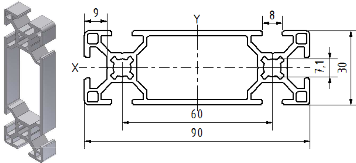
Profile 30x90 6N B-Type slot 8
