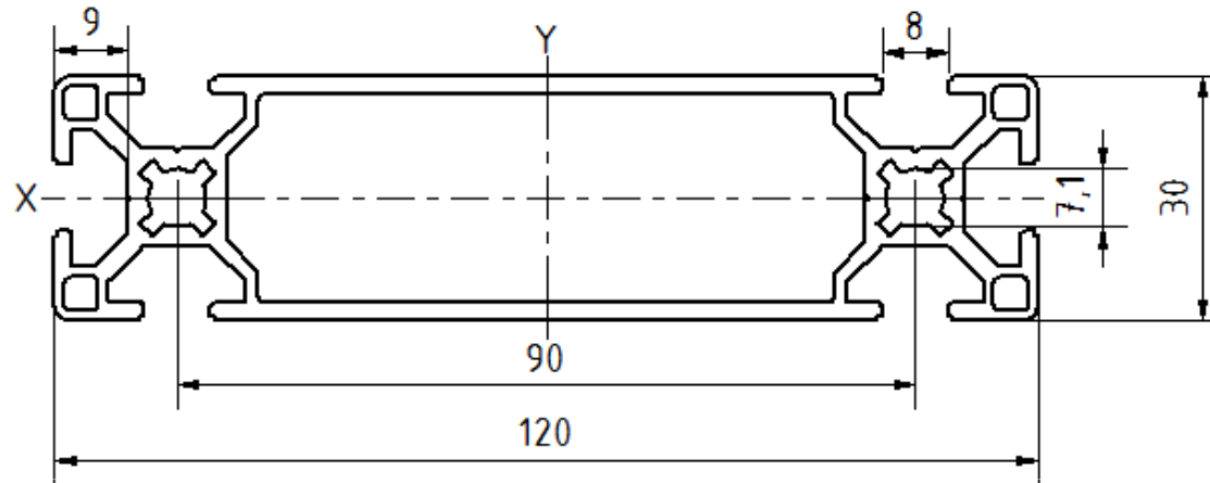
Profile 30x120 6N B-Type slot 8
