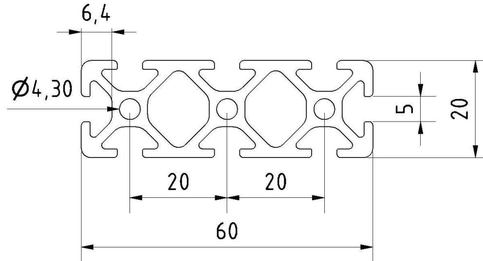
Profile 20x60 I-Type slot 5
